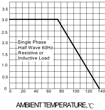
FIG.2 – FORWARD DERATING CURVE
