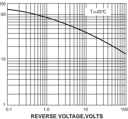
FIG. 5-TYPICAL JUNCTION CAPACITANCE
