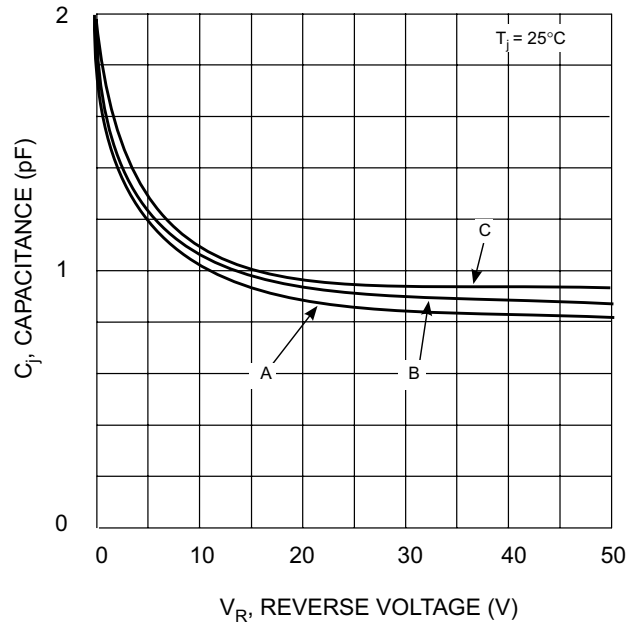
T_j = 25^\circ\text{C} V_R , REVERSE VOLTAGE (V) Fig. 2 Typ. Junction Capacitance vs Reverse Voltage
