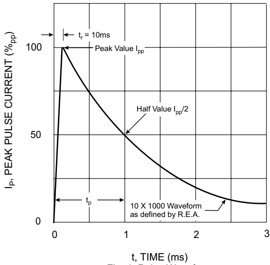
Fig. 1 Pulse Waveform
