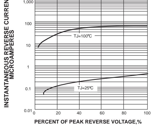
FIG. 4-TYPICAL REVERSE CHARACTERISTICS
