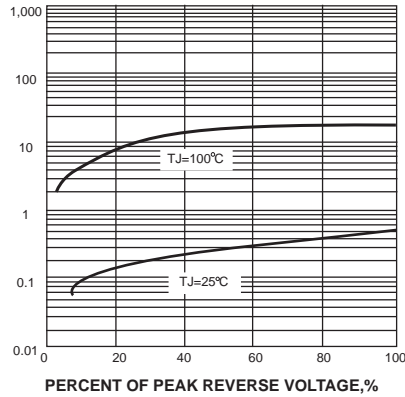
FIG. 4-TYPICAL REVERSE CHARACTERISTICS
