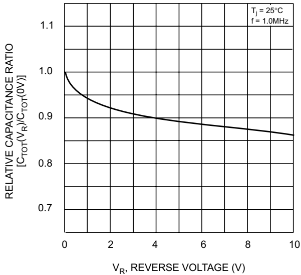
V_R , REVERSE VOLTAGE (V) Fig. 3 Relative Capacitance Variation
