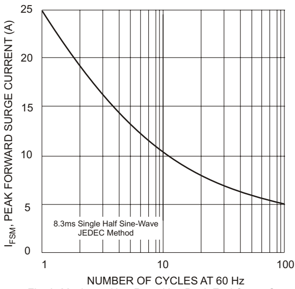
Fig. 3 Maximum Non-Repetitive Peak Fwd Surge Current
