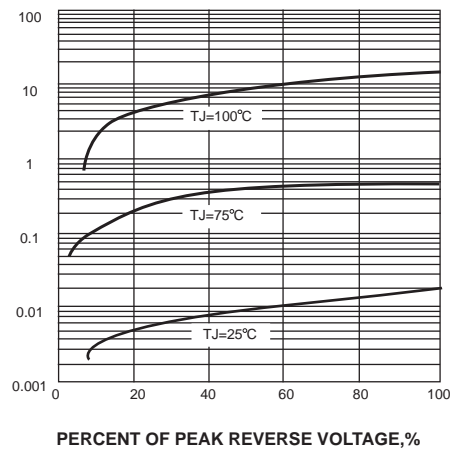
FIG. 4-TYPICAL REVERSE CHARACTERISTICS
