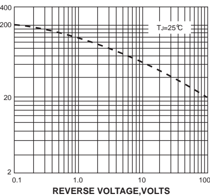
FIG. 5-TYPICAL JUNCTION CAPACITANCE
