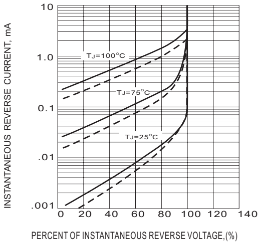
Fig.3-TYPICAL REVERSE CHARACTERISTIC
