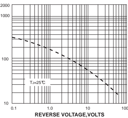
FIG. 5-TYPICAL JUNCTION CAPACITANCE
