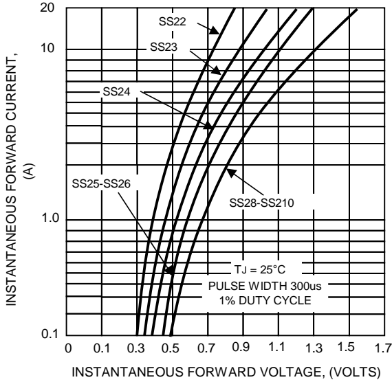
FIG.4-TYPICAL FORWARD CHARACTERISTICS
