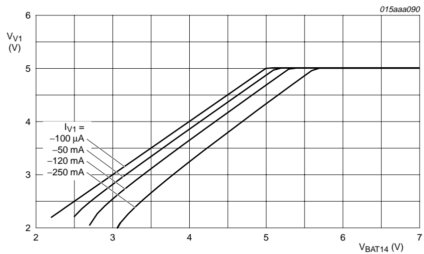
Fig 17. V 1 output voltage (dropout) as a function of battery voltage
