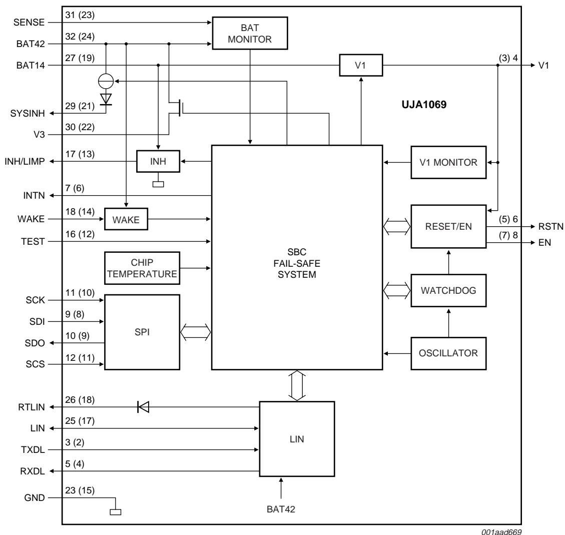
Fig 1. Block diagram
