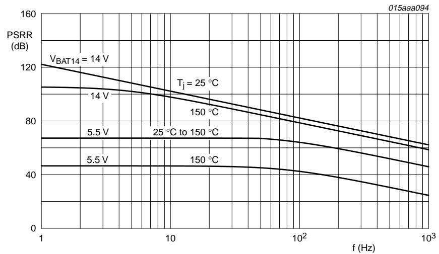
Fig 20. V1 power supply ripple rejection as a function of frequency
