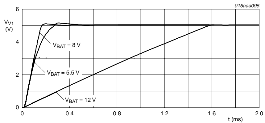
b. Behavior at T_j = 25\text{ °C}
